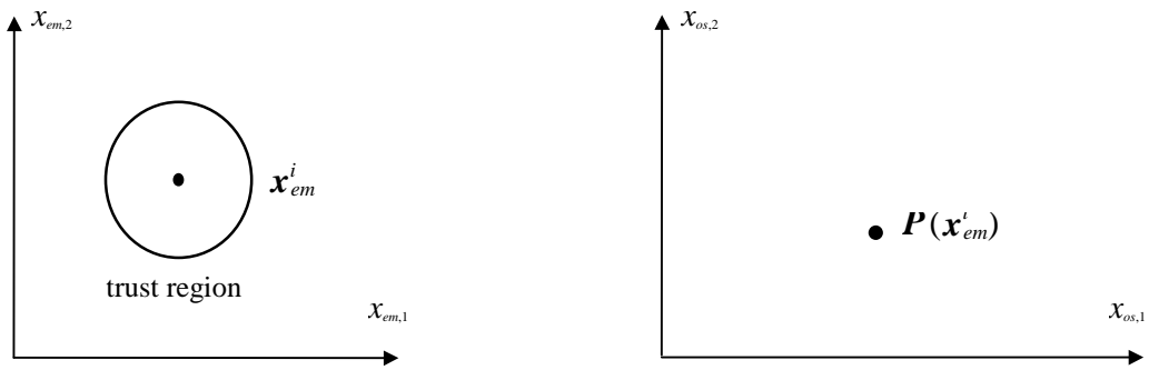
the current state at the i th iteration
