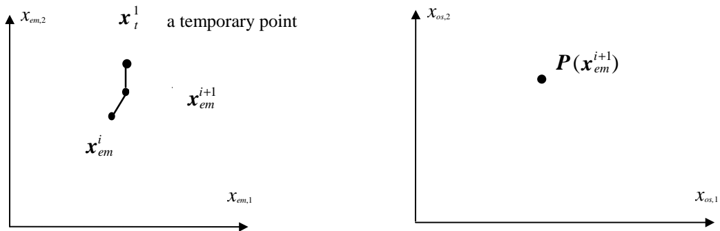
parameter extraction fails; an additional point \mathbf{x}_t^1 is obtained and multi-point parameter extraction is carried out to sharpen the solution
