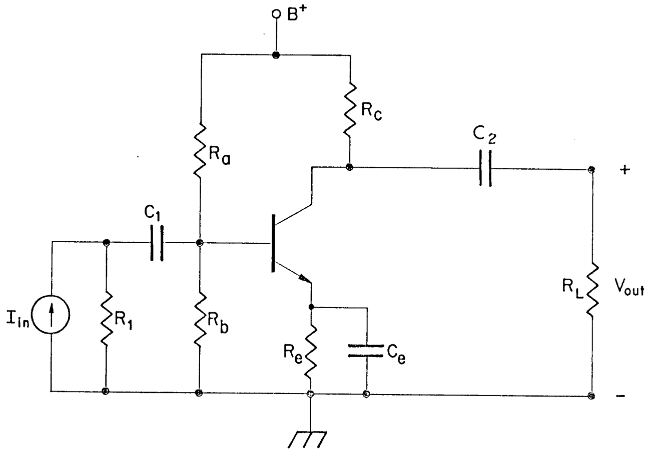
Fig. 2 The transistor amplifier circuit.
