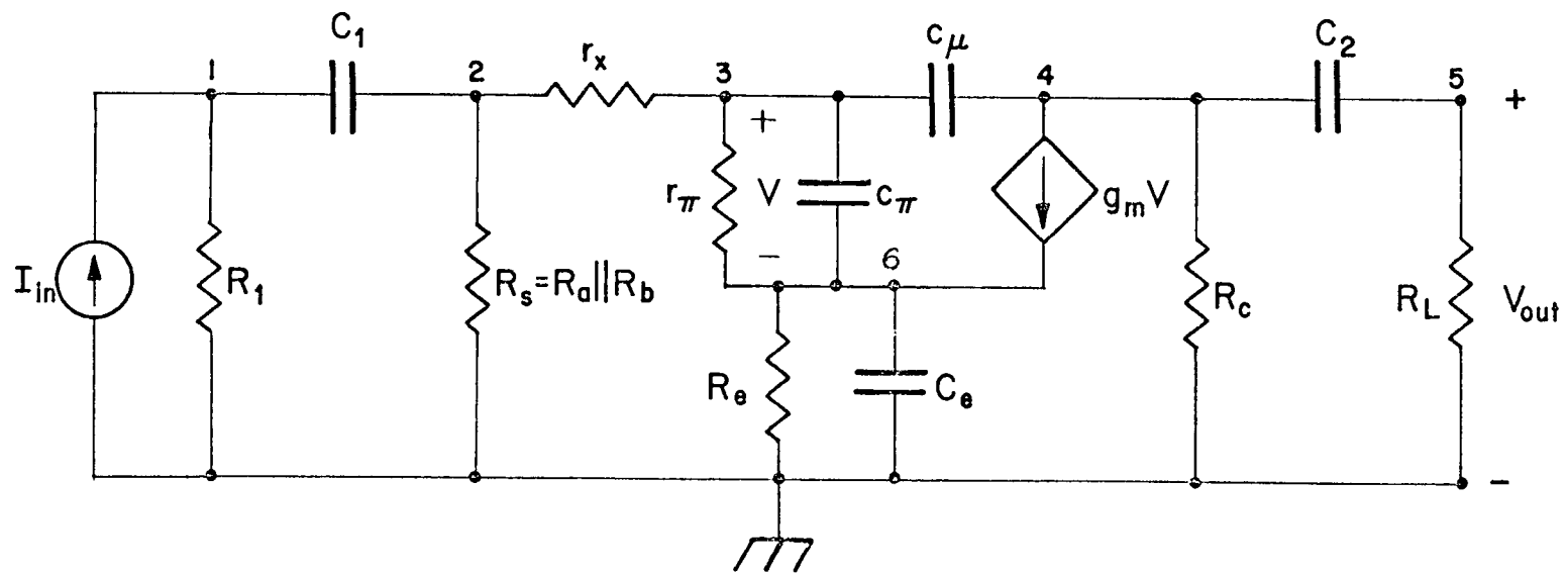
Fig. 3 The amplifier equivalent circuit.
