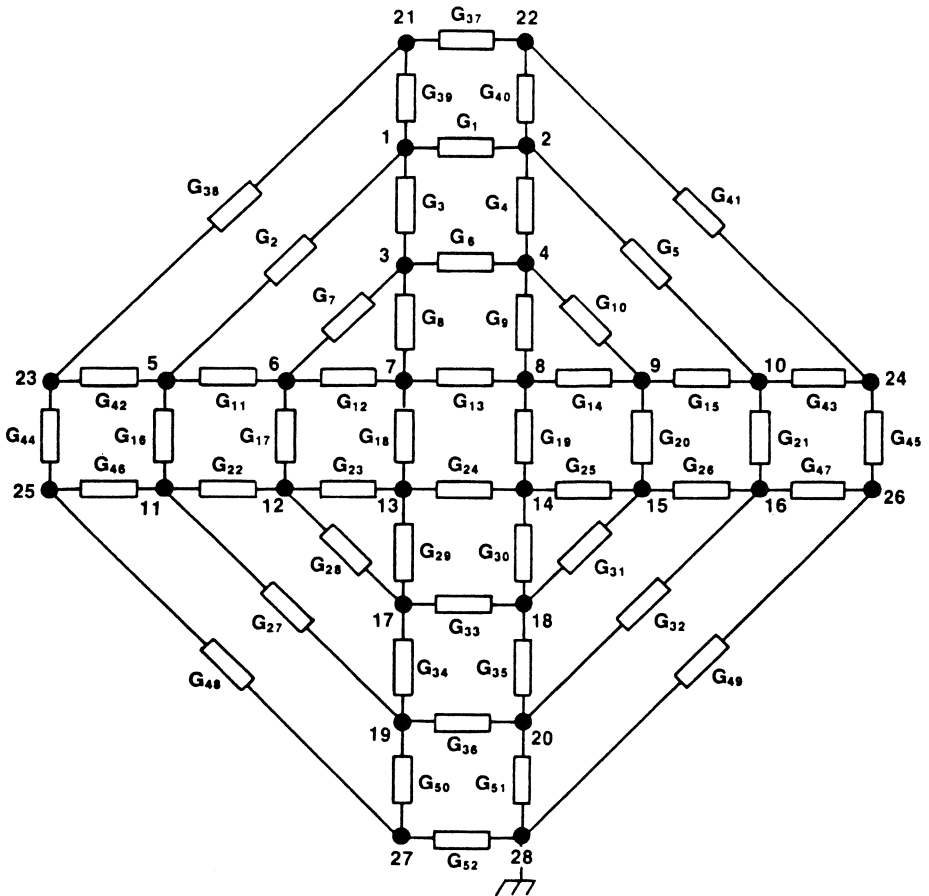
Figure 14.4 Resistive mesh network (28 nodes).
