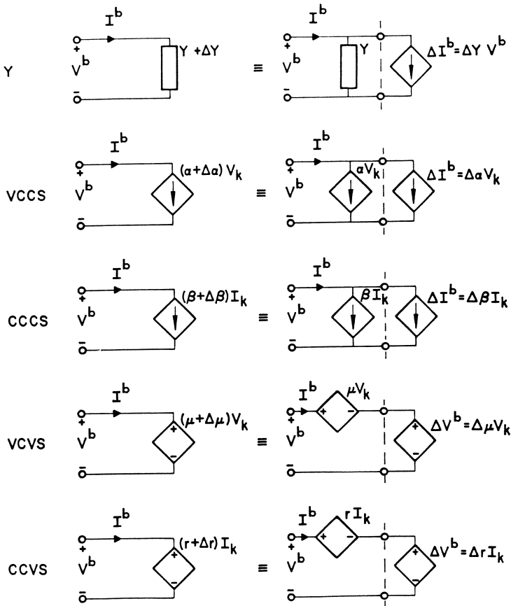
Figure 14.1 Equivalent representation of changes in element values.
