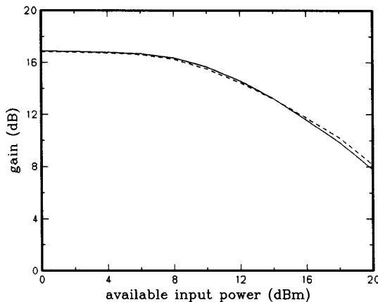
Fig. 6 Gain versus input power of the amplifier before optimization (dashed line) and after optimization (solid line).
