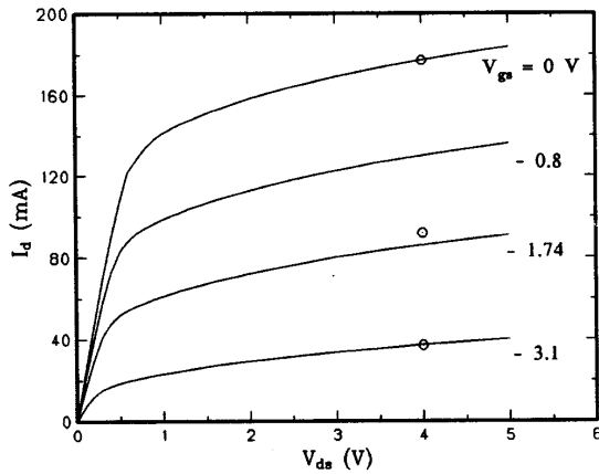
Fig. 3 DC characteristics for the parameter extraction example. The small circles indicate the measured bias points.
