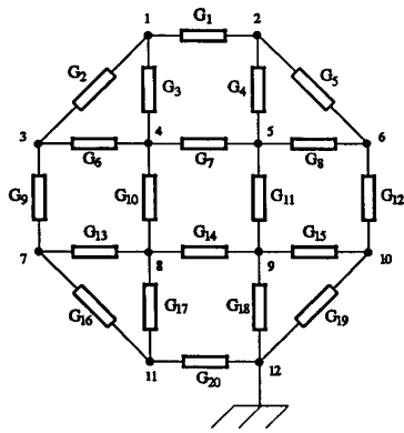
Fig. 4. The resistive mesh circuit.
