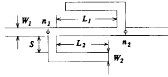
Fig. 1. Microstrip double folded stub bandstop filter [3].
