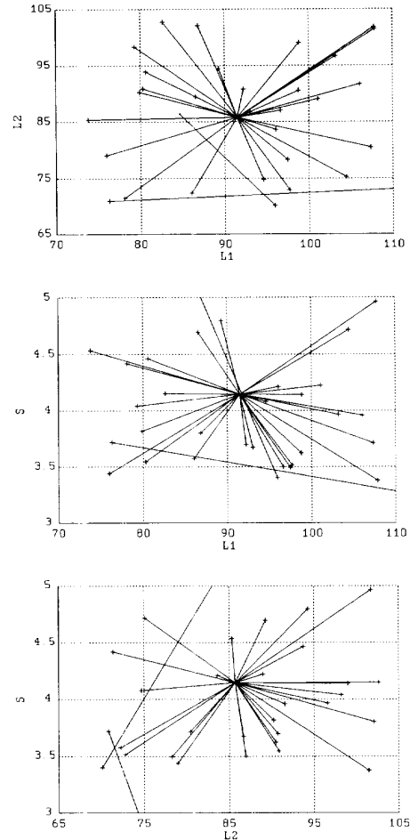
Fig. 7. Visualization of the trajectories taken by the minimax optimizer for each of the randomly generated starting points. Lines identifying corresponding starting points (+) with optimized solutions (•) for each optimization are shown in two-dimensional subspaces of the designable parameters: L_1 , L_2 and S .
