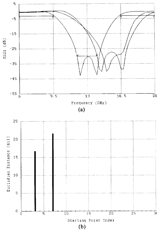
Fig. 6. (a) Simulated |S_{21}| at the optimized solutions from the 30 randomly generated starting points shown in Fig. 5, (b) the Euclidian distances between the optimized points and the reference minimax solution.
