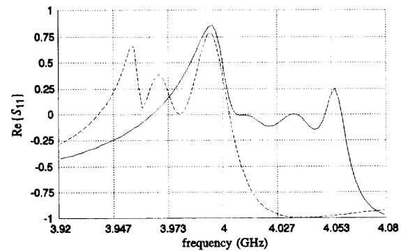
Fig. 5. \text{Re}\{S_{11}\} simulated using the empirical model (—) and em (---) at the starting point for parameter extraction.
