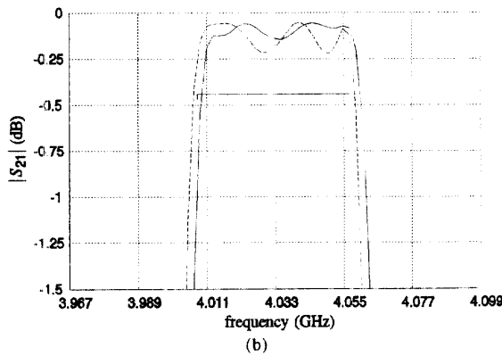
Fig. 4. The em simulated |S_{21}| response of the HTS filter at the solution obtained using the new SM optimization method (—). The OSA90/hope empirical solution (---) is shown for comparison. Responses for (a) the overall band and (b) the passband in more detail.
