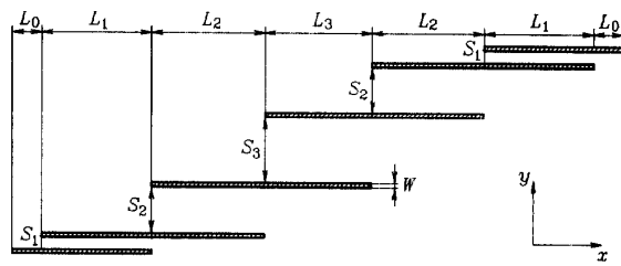
Fig. 2. The structure of the HTS filter.
