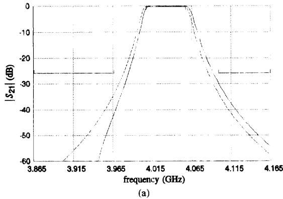
Fig. 3. The optimal |S_{21}| responses obtained using OSA90/hope (—) and the corresponding em simulation results (---).
