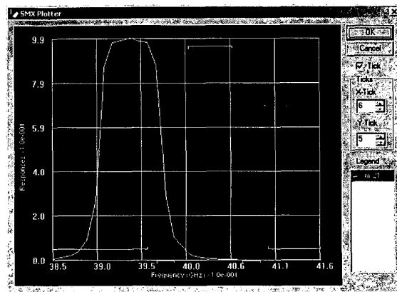
Fig. 3. Case 1: The initial response for the “fine” model (OSA90).
