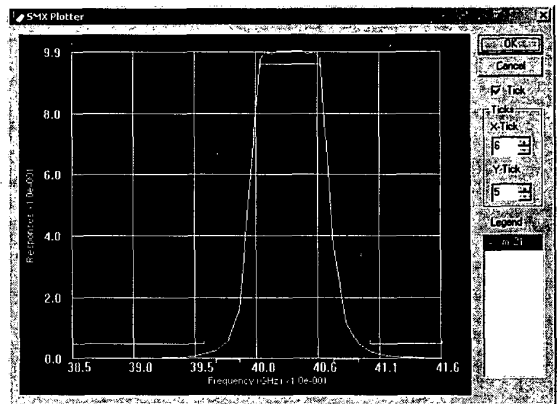
Fig. 4. Case 1: The optimal “fine” model (OSA90) response.
